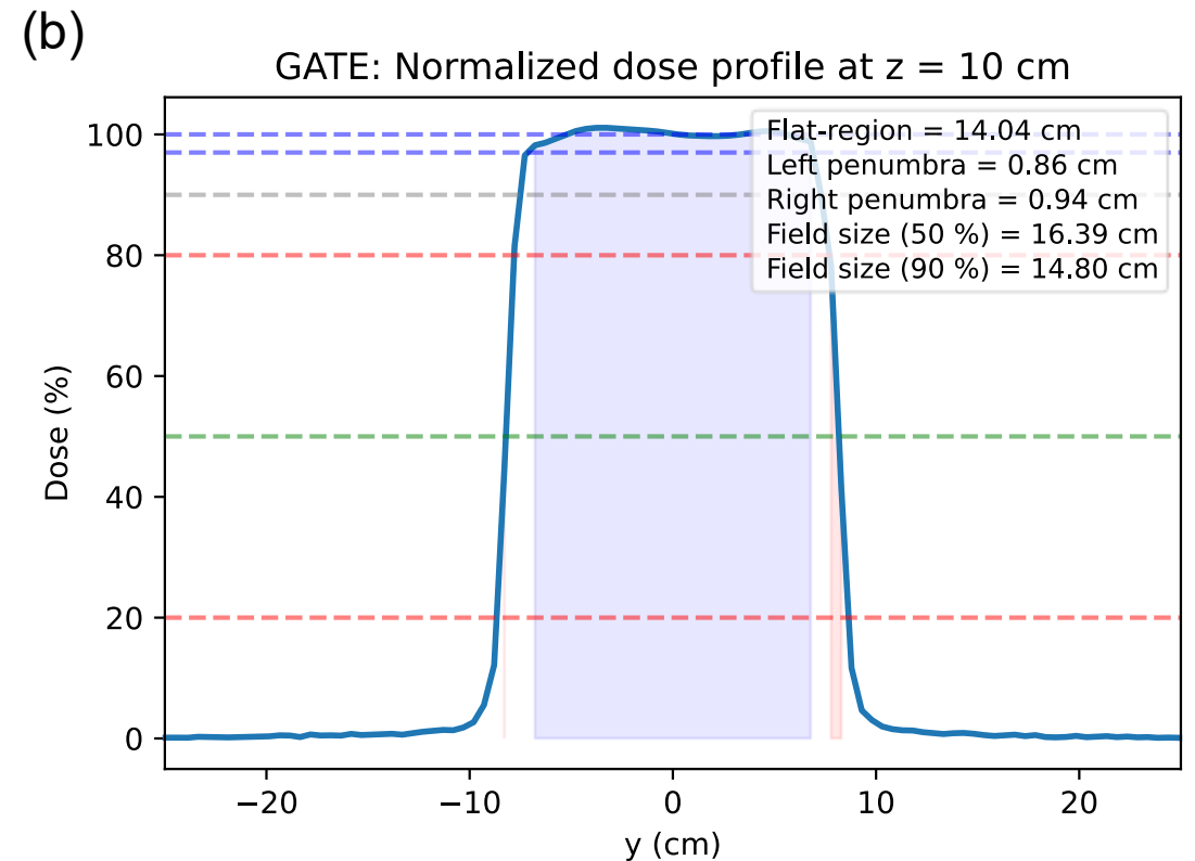
Figure 1: Comparison of lateral dose profiles at 10 cm depth for a 145 MeV VHEE beam between the (a) matRad Hong dose engine developed in this work and (b) GATE Monte-Carlo simulations with similar beam delivery system and parameters.
